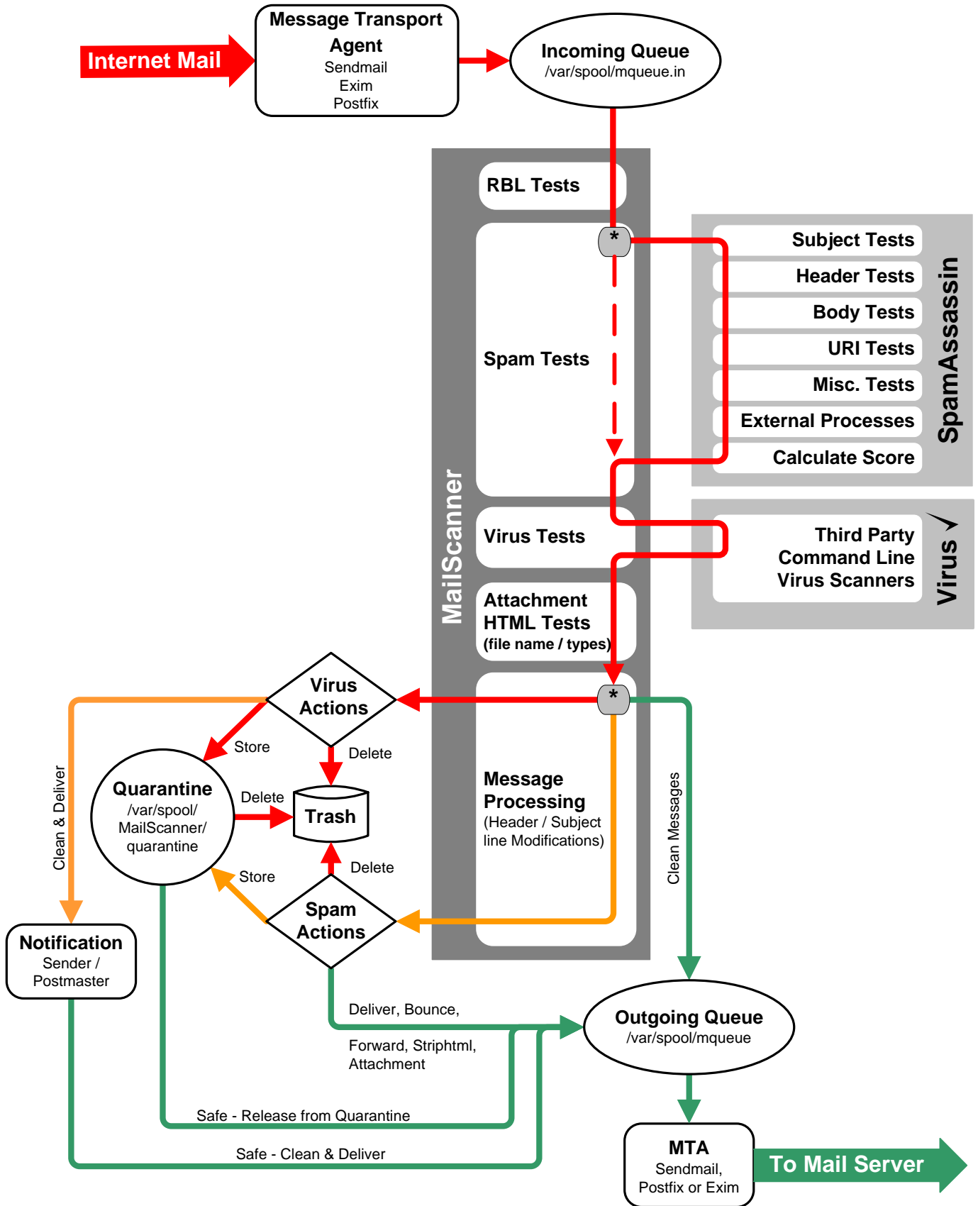
Fig. 1 MailScanner Process Flow
