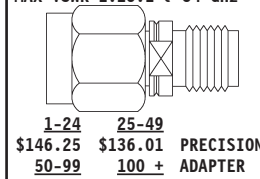
Model No. PE9650 2.4mm MALE TO 3.5mm FEMALE MAX VSWR 1.25:1 @ 34 GHz
