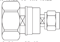
Model No. PE9637 7/16 MALE TO TNC MALE
