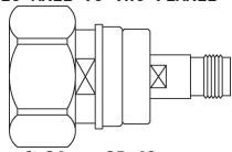
Model No. PE9636 7/16 MALE TO TNC FEMALE
