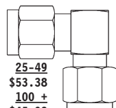
Model No. PE9642 SMA MALE TO SMA MALE RIGHT ANGLE MAX VSWR 1.35:1 @ 27 GHz
