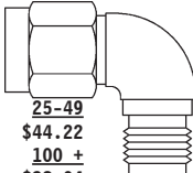
Model No. PE9641 SMA MALE TO SMA FEMALE RIGHT ANGLE MAX VSWR 1.35:1 @ 27 GHz
