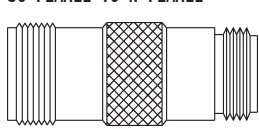
Model No. PE9292 SC FEMALE TO N FEMALE
